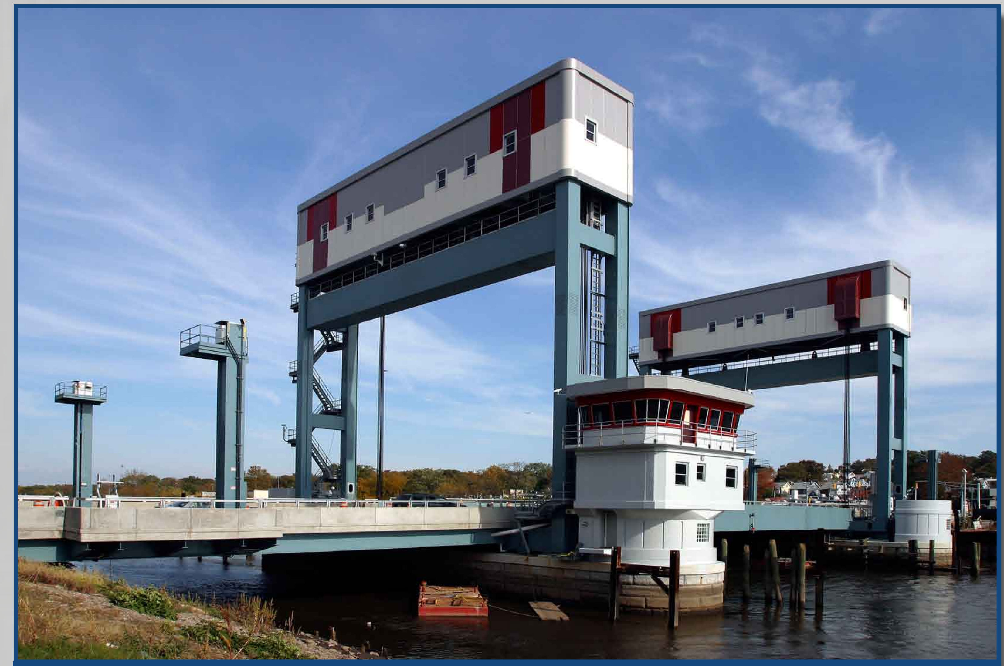
Route 7 Lift Bridge, Newark, NJ
